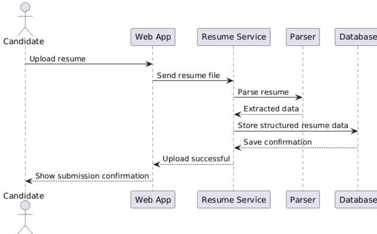
Sequence Diagram - Ali Benrami
