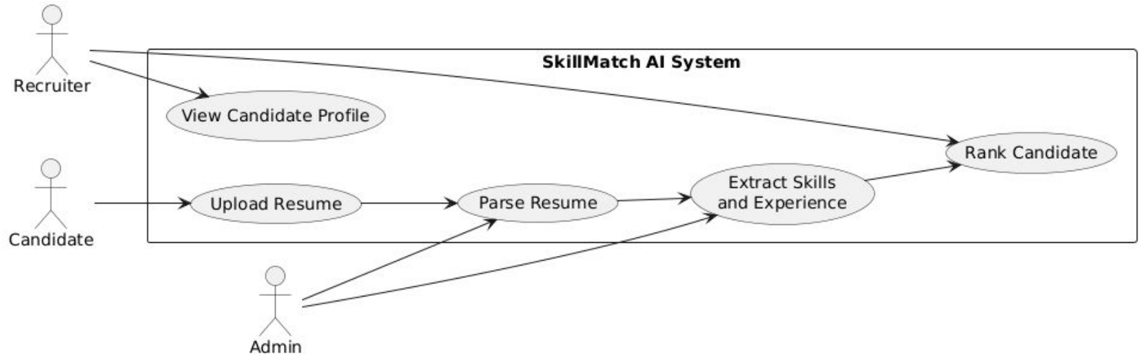
Use Case Diagram - Ali Benrami
